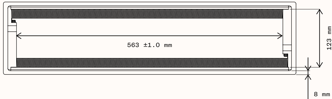
SIDE VIEWS
