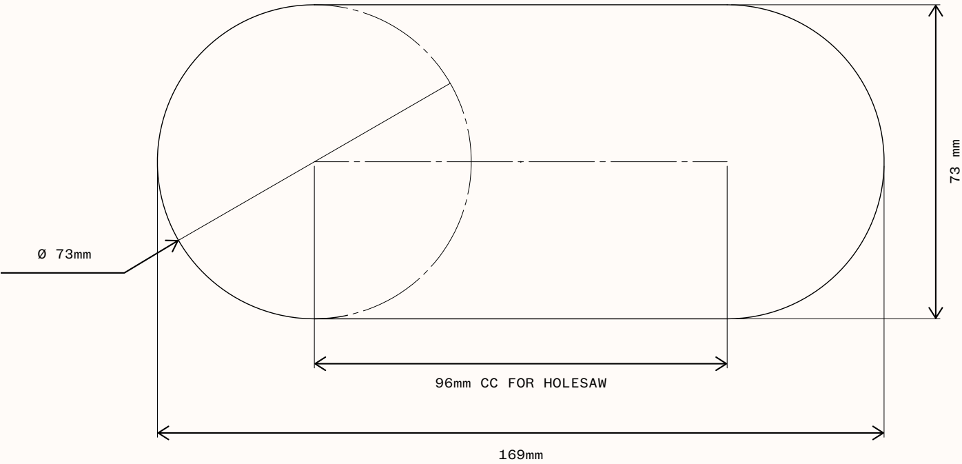
HOLE CUT DIMENSIONS
